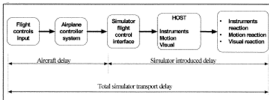
Figura 1-IIE Transport delay for simulation of computer controlled aircraft using software emulation of airplane boxes
