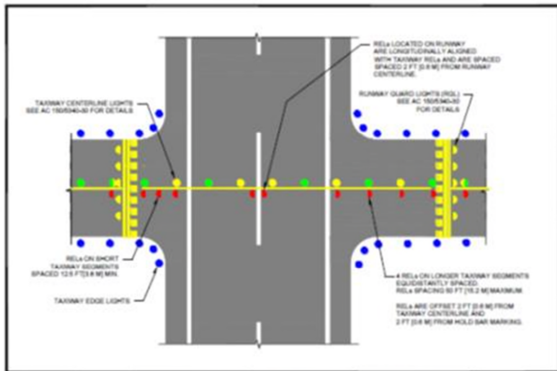
Figure 144. REL Configuration for Taxiways at 90 Degrees
